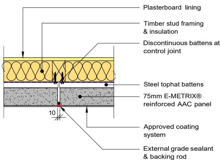
Figure 17 – Vertical control joint detail
