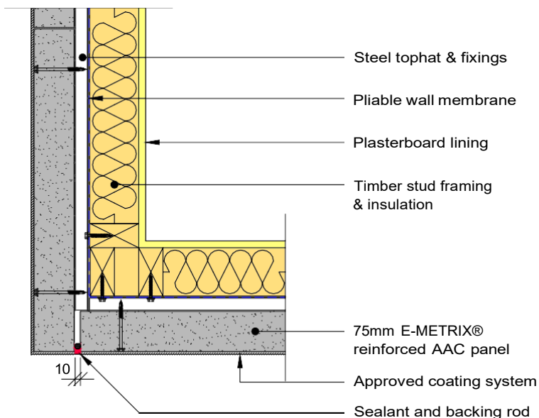
Figure 20 – External corner control joint detail
